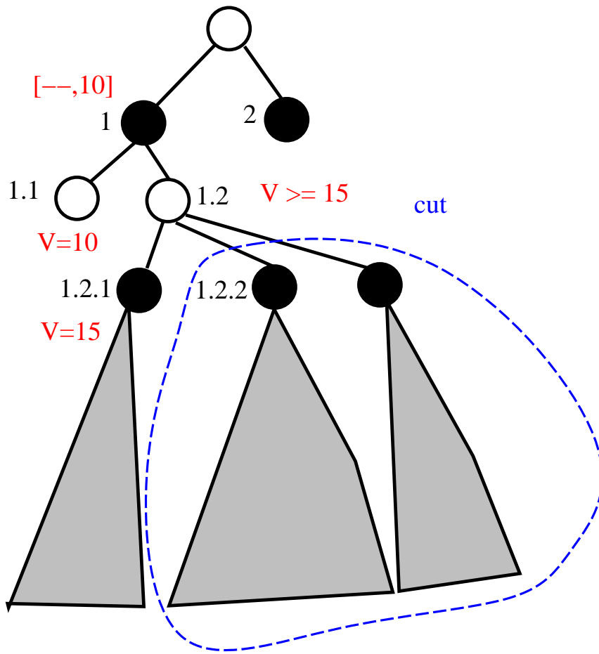
alpha-beta prune
