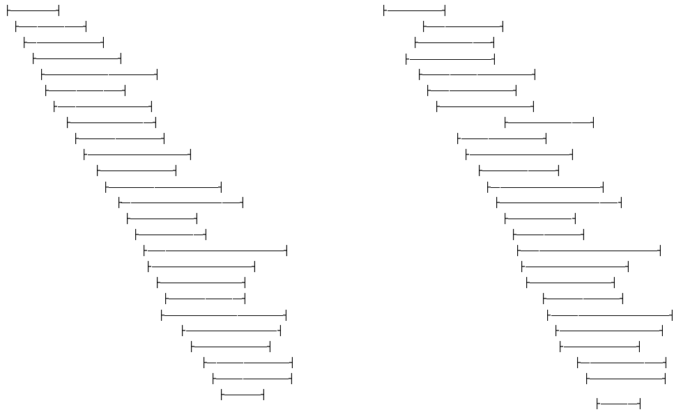
Figure 5.1 An interval graph with 25 intervals at error rate 5%
