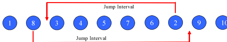
Figure 5.1. An example of jump intervals.
