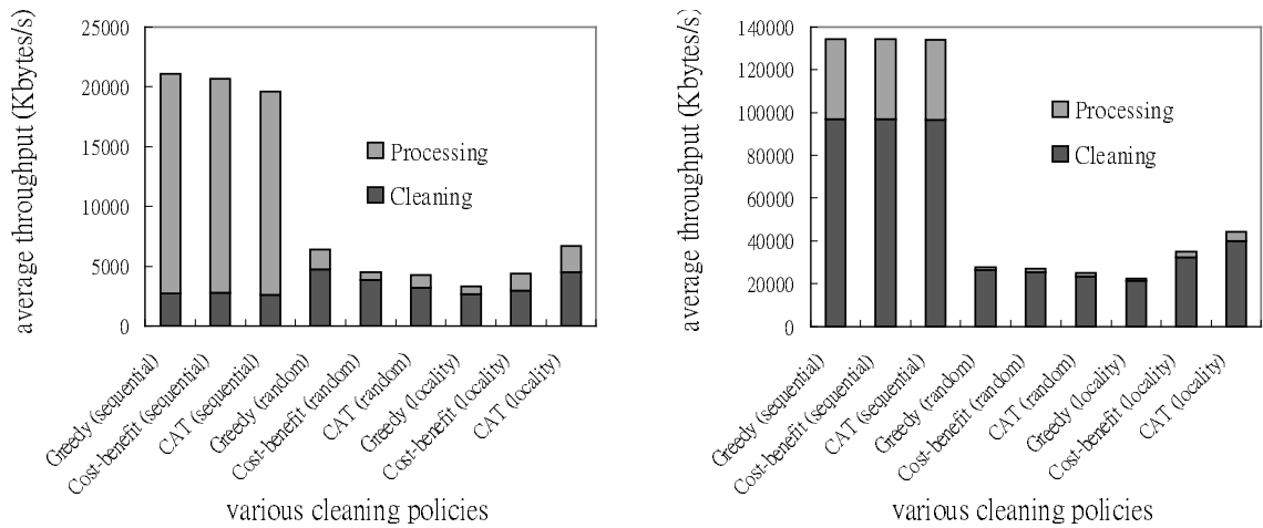
(a) Intel 486 DX 33.
