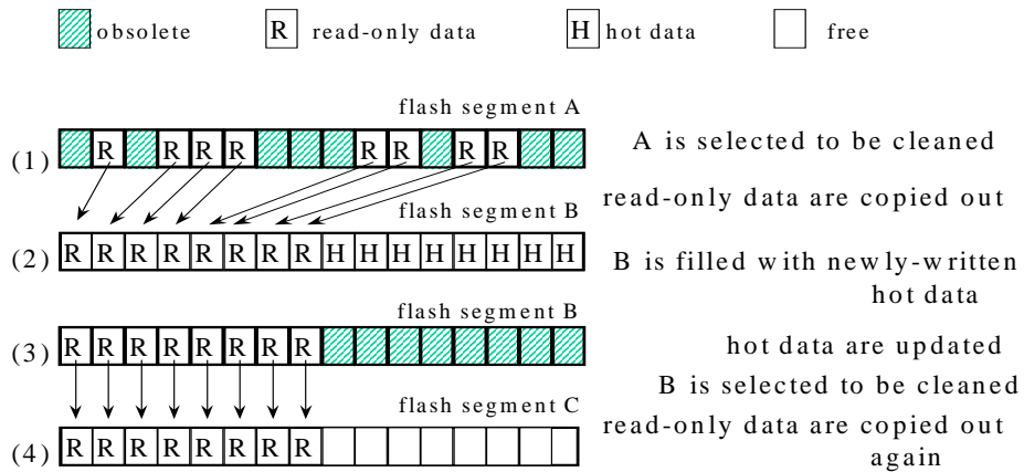
Figure 4: Repeatedly migrating read-only data when they are mixed with dynamic data.
