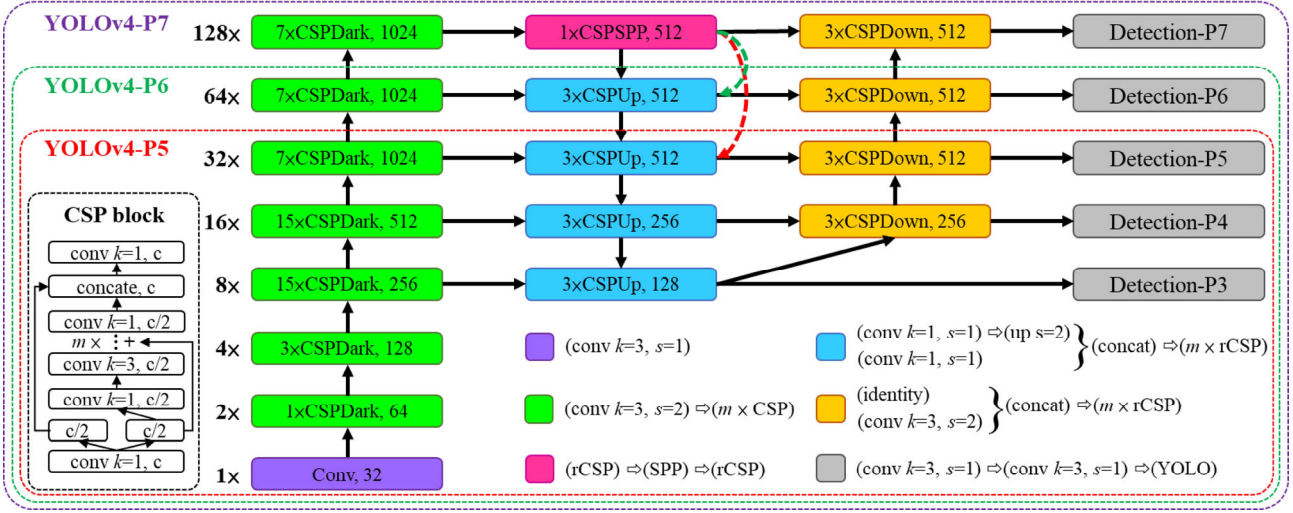
Figure 4: Architecture of YOLOv4-large, including YOLOv4-P5, YOLOv4-P6, and YOLOv4-P7. The dashed arrow means replace the corresponding CSPUp block by CSPSPP block.
