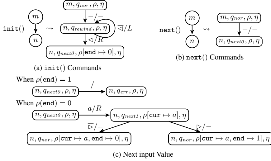
Fig. 5: Construction of A_G (continued)
