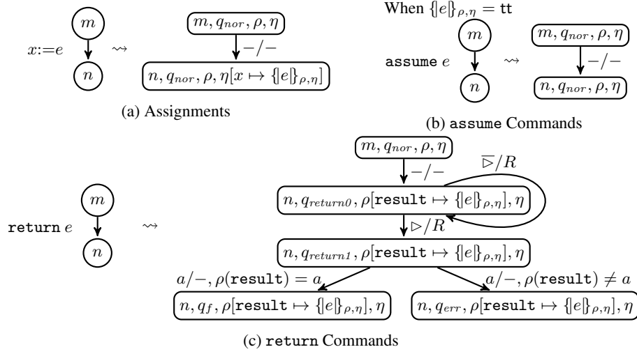
Fig. 4: Construction of A_G
