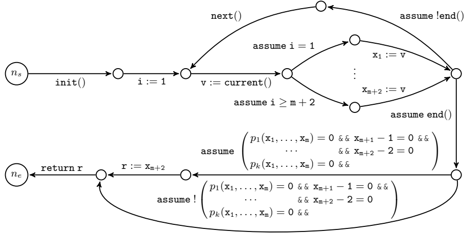
Fig. 2: A Single-Pass Integer Reducer
